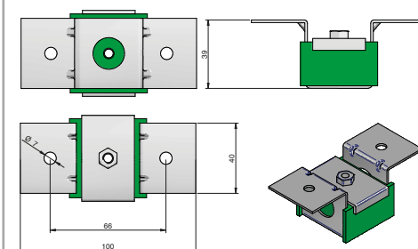
Akustik 1 Lateral + Sylomer ® (Standard position)
