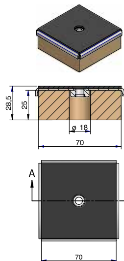
TSR with a levelling kit.
