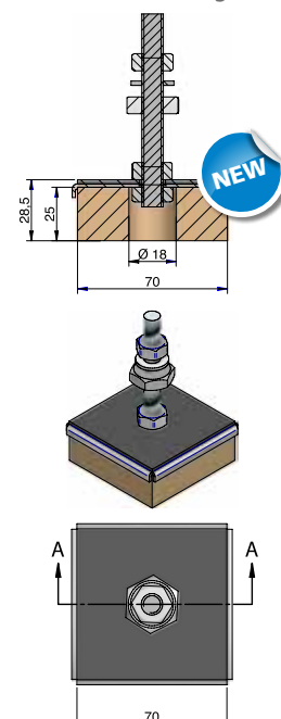
TSR with a levelling kit.
